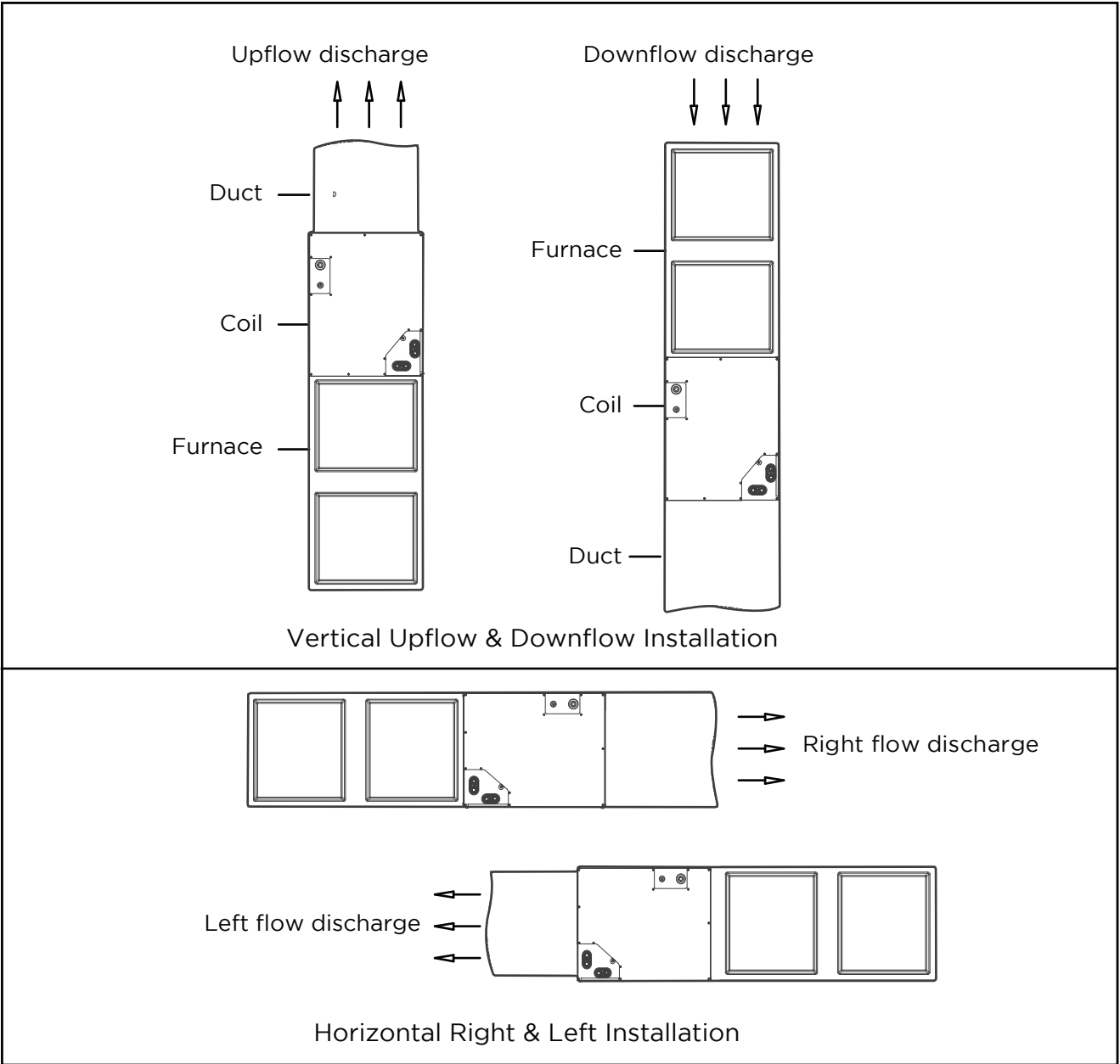
Installation type 2: Model SENDC-60CO-C coil installation on furnace
